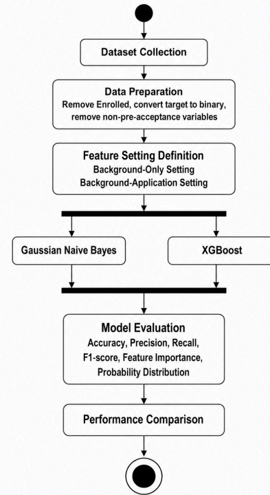
Fig. 1. Research workflow of the proposed pre-acceptance student dropout prediction framework.
