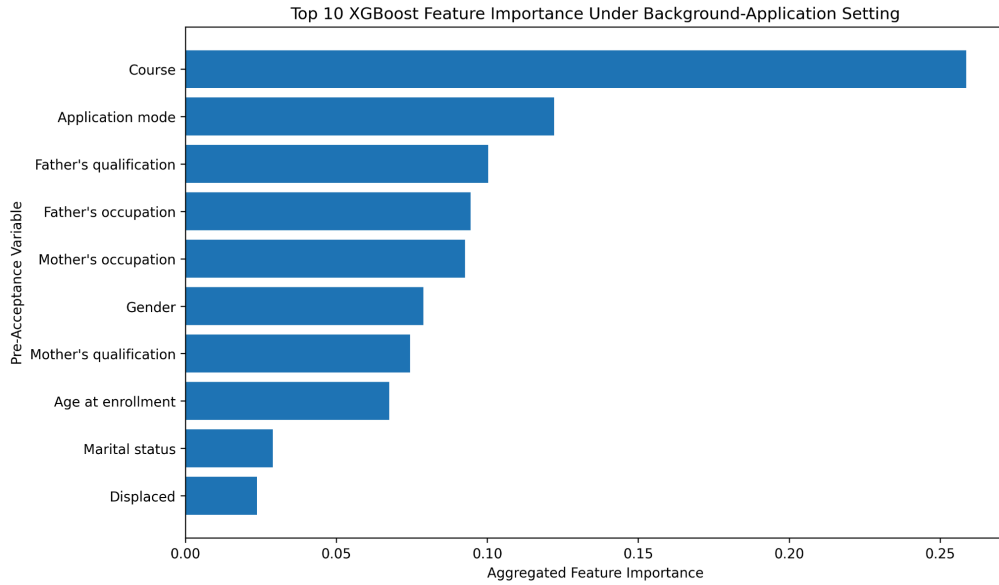
Fig. 2. Top 10 XGBoost Feature Importance Under Background-Application Setting
