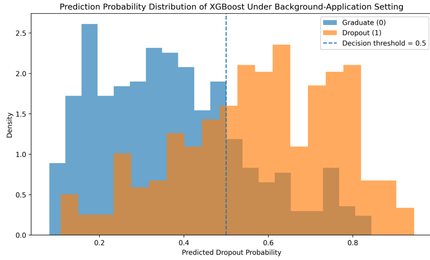
Fig. 3. Prediction Probability Distribution of XGBoost Under Background-Application Setting
